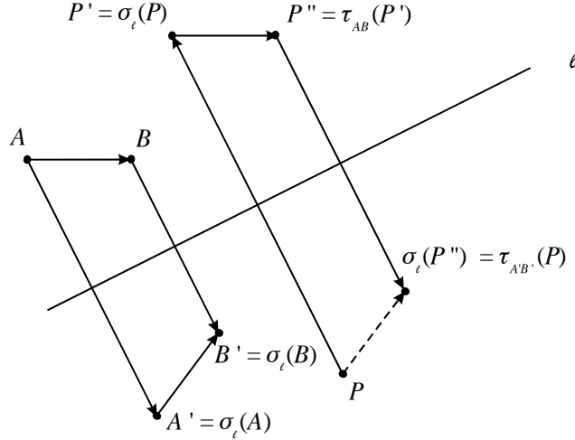
Figure 3.8: Conjugation of \tau_{AB} by \sigma_\ell .
